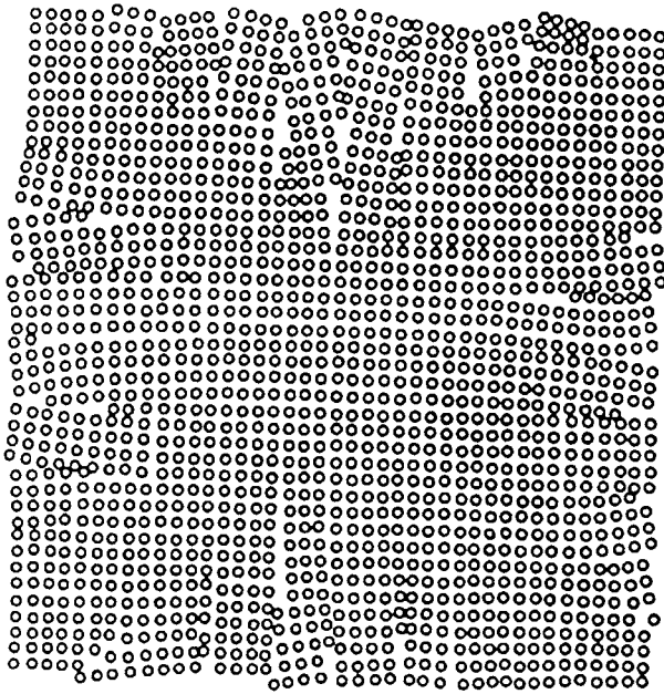
Figure 6.1. Polycrystals.
