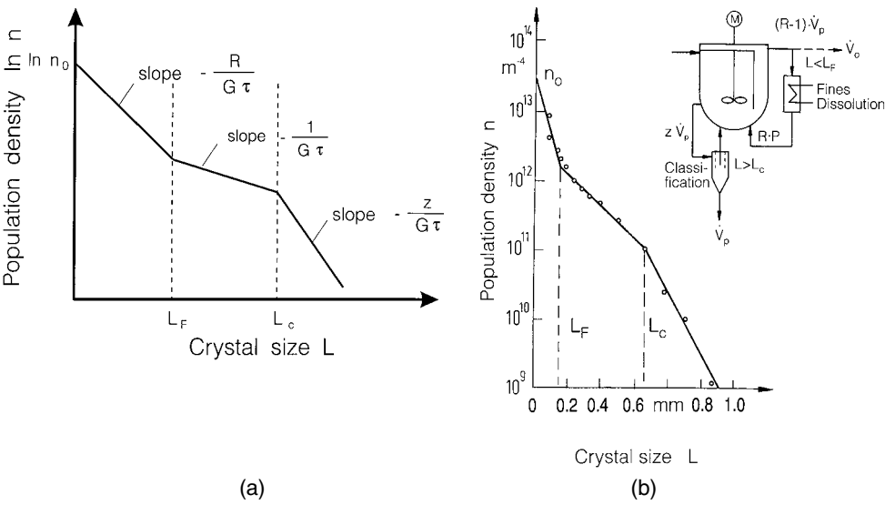
Figure 5.2. Population density versus crystal size for fines destruction and classified product removal: (a) principal; (b) experimental.
