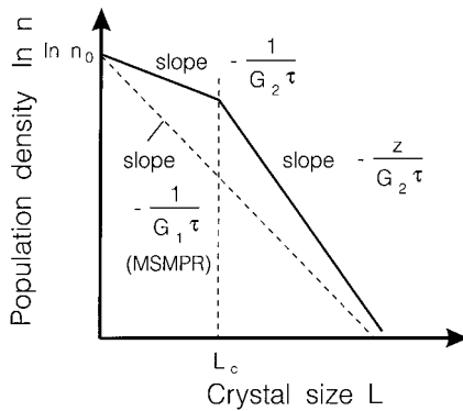
Figure 6.2. Population density versus crystal size for classified product removal.
