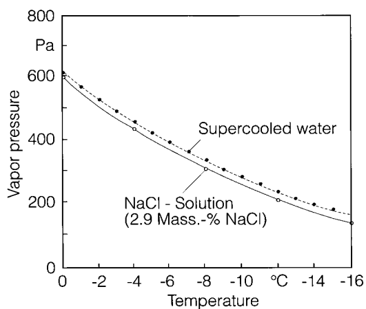
Figure 2.13. Vapor pressure of \text{H}_2\text{O} and \text{NaCl-H}_2\text{O} versus the temperature.
