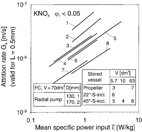
Figure 3.3. Attrition rate (valid for L = 0.5 mm) against the mean specific power input for stirred-vessel and FC crystallizers.
