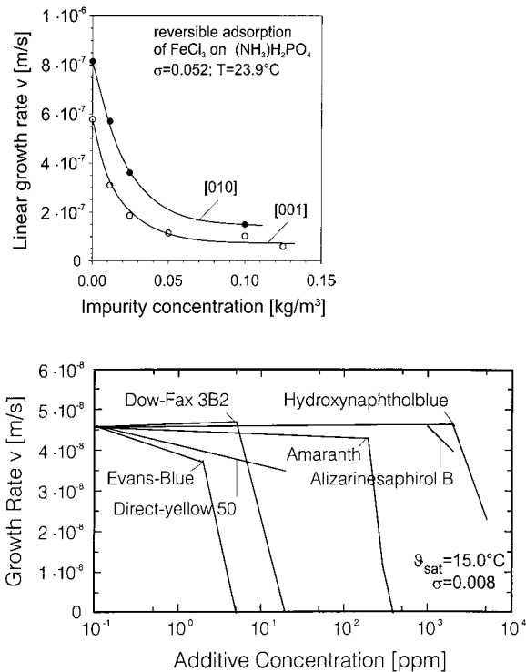
Figure 5.4. Nonzero and zero growth behavior as a consequence of reversible and irreversible adsorption of impurities. (a) Reversible adsorption of FeCl 3 and AlCl 3 on the [001] and [010] directions for the {100} faces of (NH 3 )H 2 PO 4 [5.3]; (b) irreversible adsorption of various additives on the {110} face of KNO 3 [5.23].
