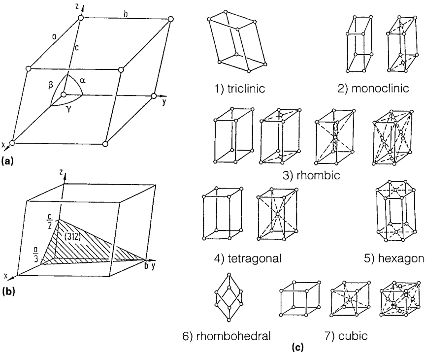
Figure 4.1. (a) Elementary cell (upper left); (b) explanation of Miller's index; (c) different crystal systems.
