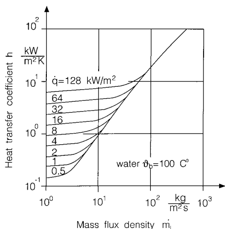
Figure 8.4. Mean heat transfer coefficient versus mass flux density when water boils at 1 bar.
