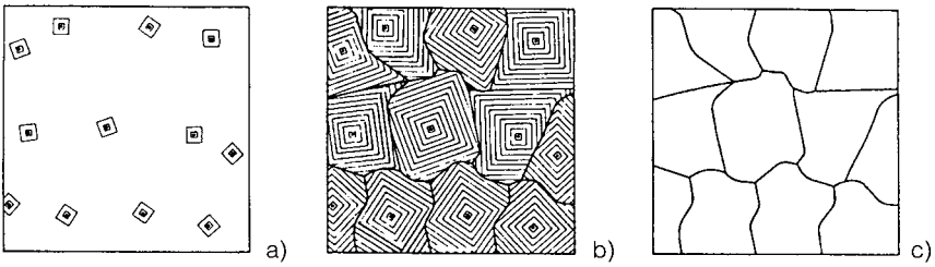
Figure 6.3. Formation of polycrystals.
