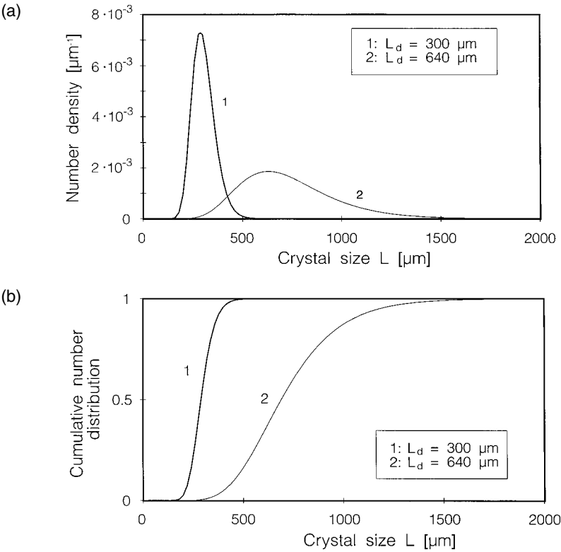
Figure 1.2. Density (population and mass) and cumulative undersize population and mass against crystal size L .
