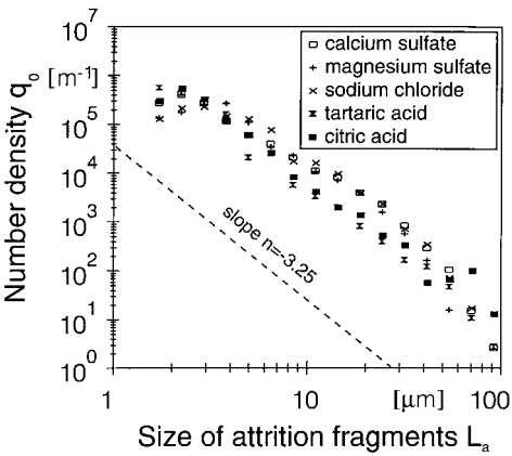
Figure 1.10. The number–density distribution of fragments generated. (From Ref. 1.16.)
