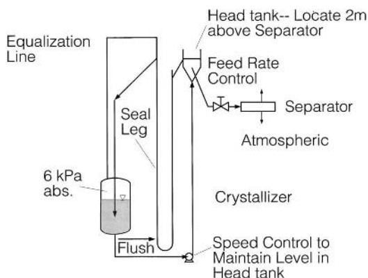
Figure 7.4. Slurry transportation system with change of the pump speed.
