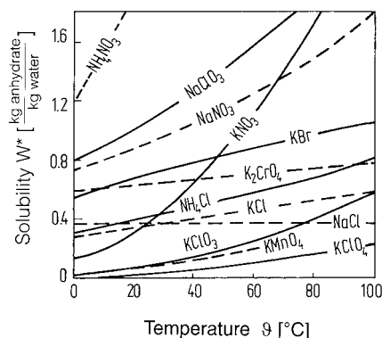
Figure 2.1. Solubility curves for several anhydrides.
