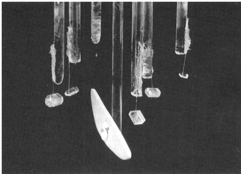
Figure 6.1. Three (D) and three (L) crystals of asparagine- \text{H}_2\text{O} grown together for 45 days under conditions close to equilibrium in the presence of (L)-serine; the large crystals are (D)-Asn- \text{H}_2\text{O} and the small ones are (L)-Asn- \text{H}_2\text{O} .
