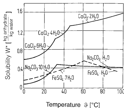
Figure 2.2. Solubility curves for several hydrates.
