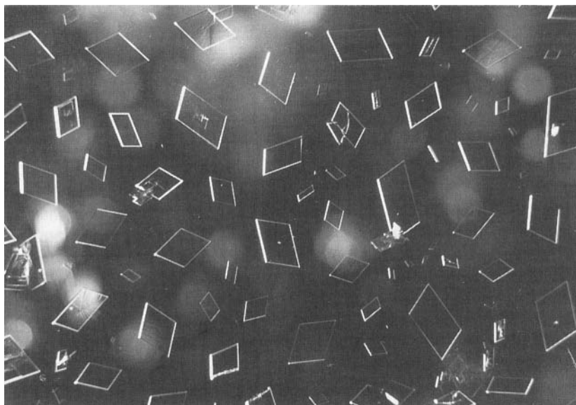
Figure 6.3. Floating crystals of \alpha -glycine grown in the presence of 1% wt/wt (L)-leucine and 3% (D,L)-glutamic acid, exposing their (010) face to air.
