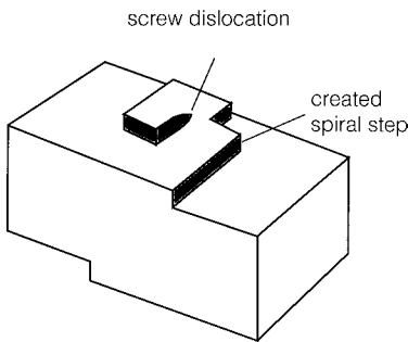
Figure 6.6. A screw dislocation and a created spiral step.
