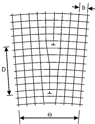
Figure 6.7. A simple tilt boundary.
