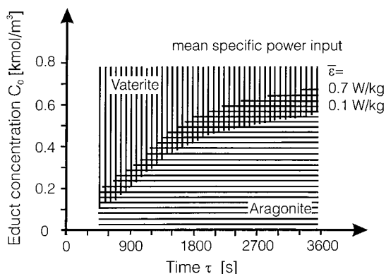
Figure 5.1. Polymorphism of calcium carbonate with residence time, concentrations of reactants, and mean specific power input as parameters.
