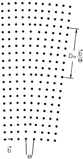
Figure 6.4. Grain boundary due to a small angle.
