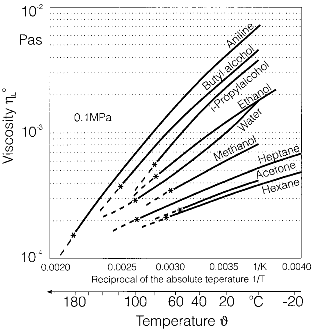
Figure A1.2. Dynamic viscosity \eta_L^\circ versus the temperature for some solvents.
