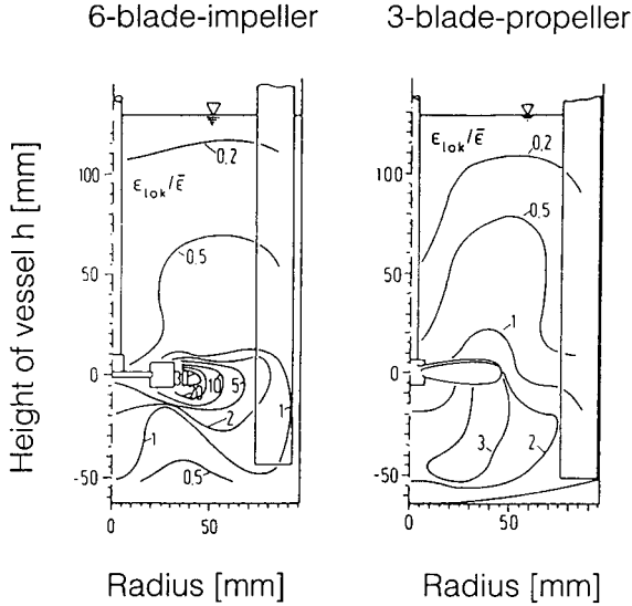
Figure 5.2. Lines of constant energy dissipation \varepsilon/\bar{\varepsilon} for different stirrers in water. (From [3.10].)
