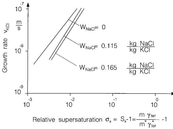
Figure 4.4. Growth rate of KCl against supersaturation.
