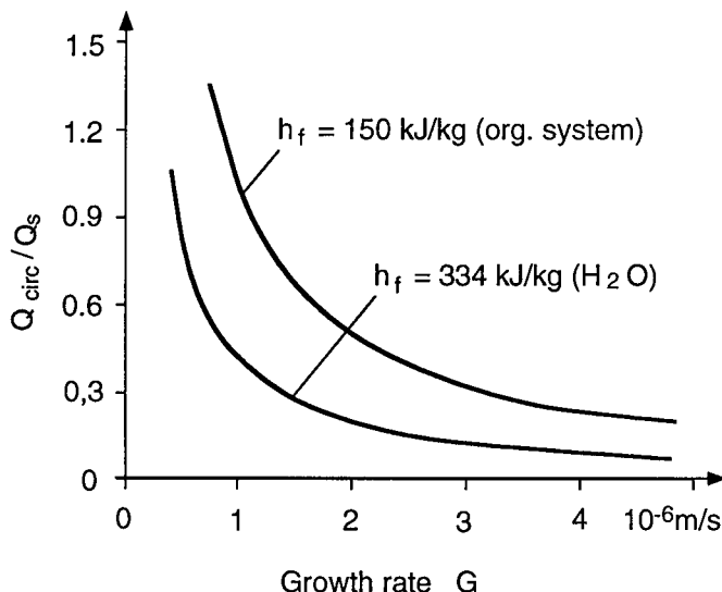
Figure 1.13. Energy input for the melt circulation as a function of the growth rate of the crystalline layer; \delta_s = 0.008 m.
