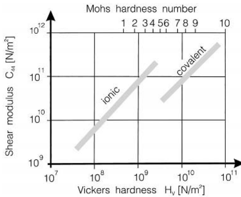
Figure 7.6. Shear modulus C_{44} against Vickers hardness.
