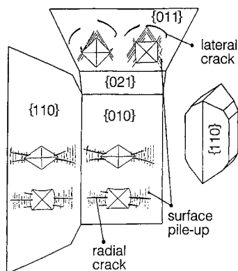
Figure 7.4. Illustration of crack patterns and surface pileup for indentations on potassium nitrate.
