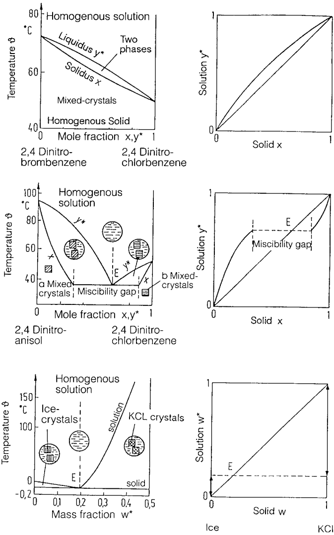
Figure 2.5. Melting and solidification curves of several systems.
