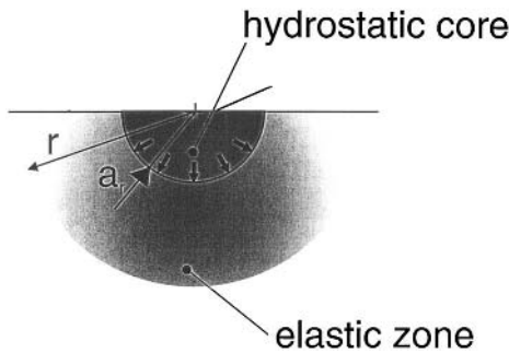
Figure 1.4. Simplified stress field created by a plastic–elastic induction. (From Ref. 1.9.)
