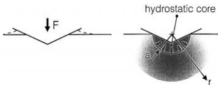
Figure 7.1. Indentation test (Vickers hardness) (left); definition of a and r (right).
