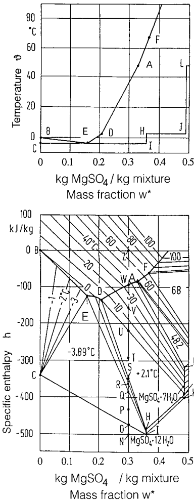
Figure 3.1. Solubility and enthalpy–concentration diagram of an aqueous magnesium sulfate solution.
