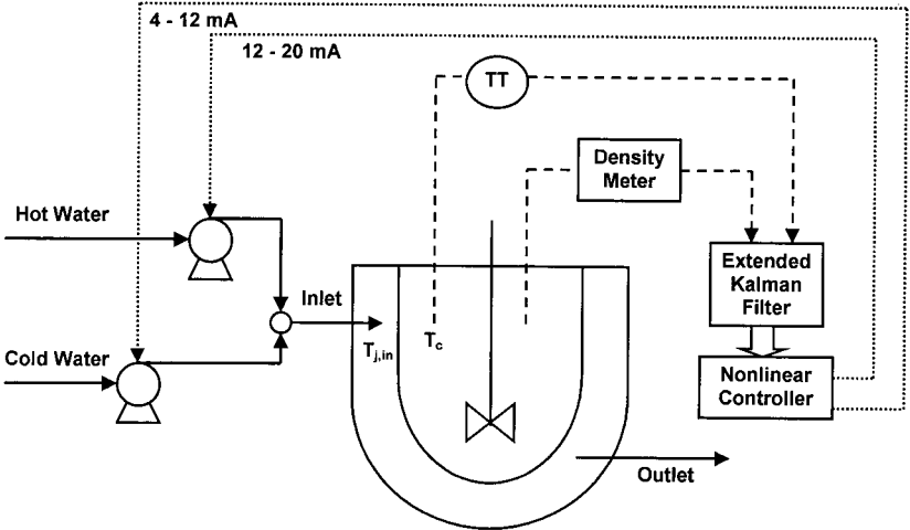
Figure 4.3. The piping and instrumentation diagram of the EKF NGC used for the control of supersaturation in a cooling batch crystallization of potash alum.
