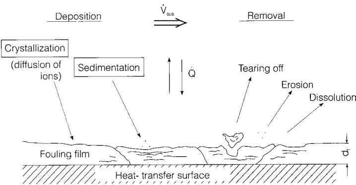
Figure 6.5. Deposition and removal processes.
