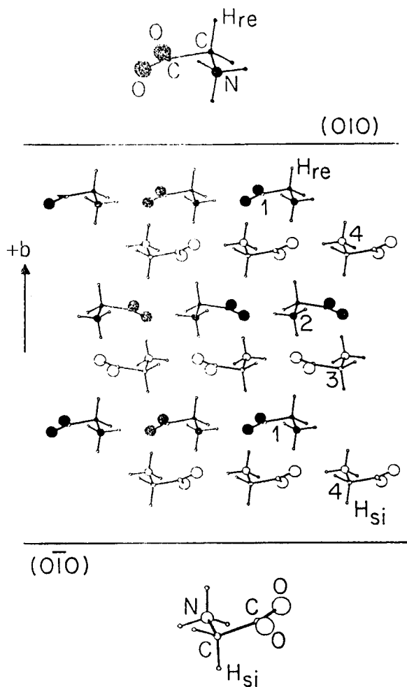
Figure 5.3. Packing arrangement of \alpha -glycine viewed along the a axis showing the four symmetry-related molecules; C— H_{re} bonds of all the molecules point toward the (010) face and the C— H_{si} bonds to the (0\bar{1}0) face.
