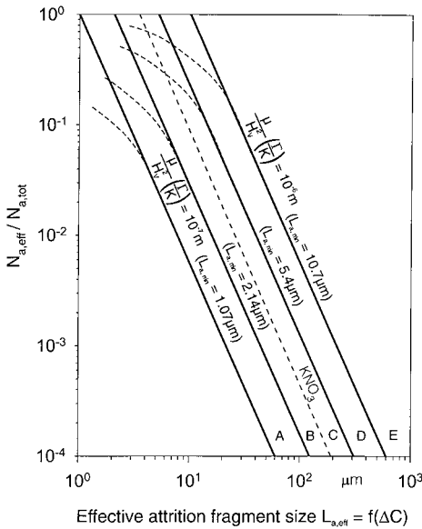
Figure 4.2. The ratio of effectively growing fragments as a function of their mechanical material properties and size.
