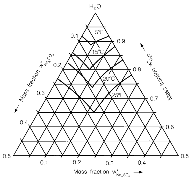
Figure 2.3. Triangular diagram of the sodium carbonate–sodium sulfate–water system.
