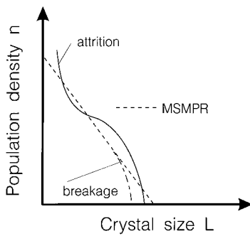
Figure 7.3. Deviation from the straight line due to mechanical effects (fluid shear and solid attrition effects).
