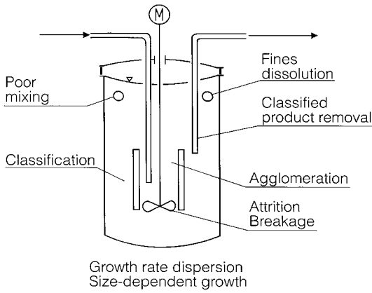
Figure 7.1. Effects in a nonideal MSMPR crystallizer.
