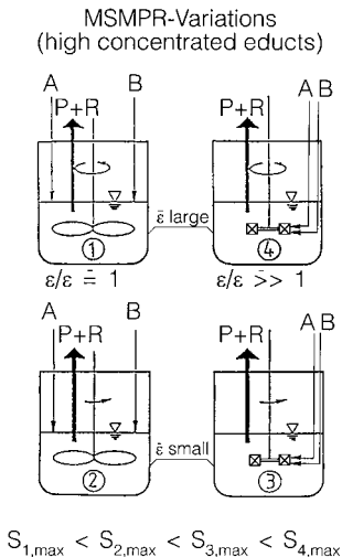
Figure 4.5. Operating modes of continuous-precipitation crystallizers.
