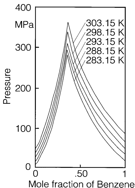
Figure 2.1. Phase diagram of the system benzene-cyclohexane.
