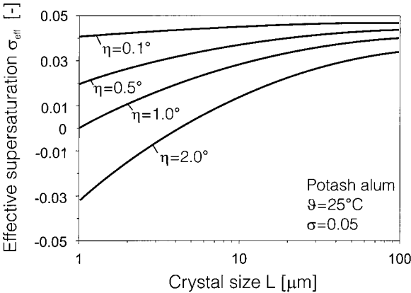
Figure 6.5. Effective relative supersaturation against the crystal size for different mosaic spreads.
