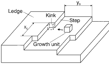
Figure 2.1. Energetically favorable sites for integration.
