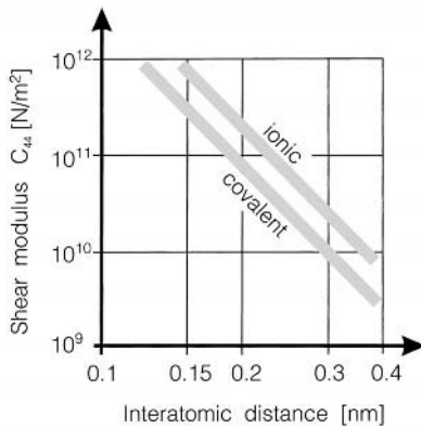
Figure 7.5. Shear modulus C_{44} against interatomic distance.
