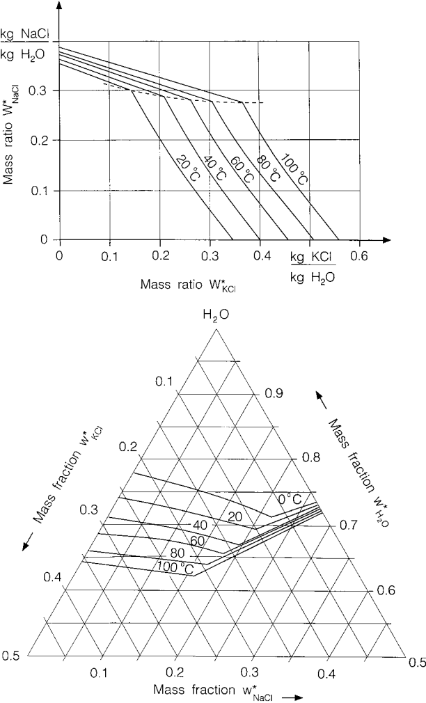
Figure 4.3. Solubility of the ternary KCl–NaCl–water system: (a) w_{\text{NaCl}}^* against w_{\text{KCl}}^* ; (b) triangular diagram.
