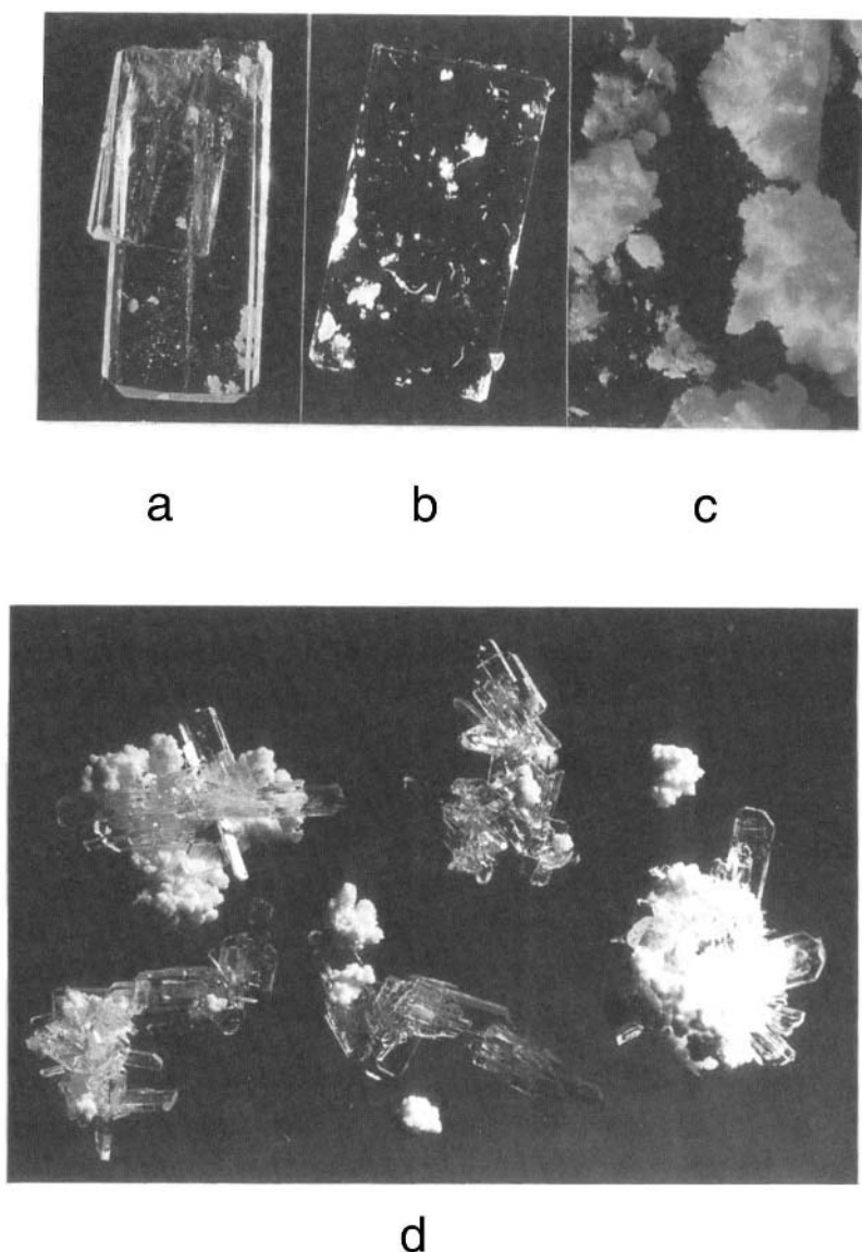
Figure 2.3. Crystals of (L)-Glu·HCl grown in the presence of an increasing amount of additive (L)-lysine: (a) no additive or (D)-lysine; (b) +2 mg/mL (L)-lysine; (c) +50 mg/mL (L)-lysine; (d) crystals of racemic Glu·HCl grown in the presence of (L)-lysine. The plates are the (D) enantiomer, whereas the powder is the (L) enantiomer.
