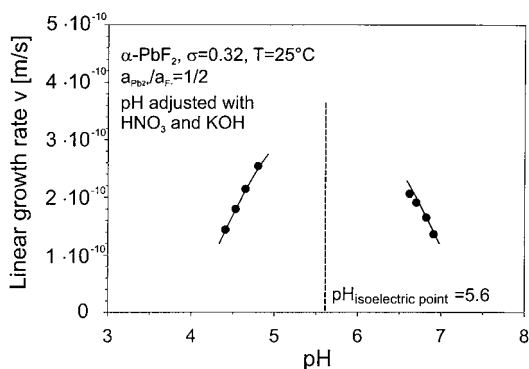
Figure 4.6. Linear growth rate of \alpha -PbF 2 at 25°C from acidic \text{pH}^\circ = 3.5 and alkaline \text{pH}^\circ = 7.1 (at positive and negative surface charge, respectively) supersaturated solution as a function of pH, \text{Pb}^{2+} , and \text{F}^- activity ratio R = \frac{1}{2} . (Data from Ref. 4.7.)
