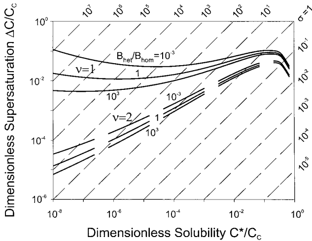
Figure 4.1. Ratios of heterogeneous to homogeneous nucleation rates.
