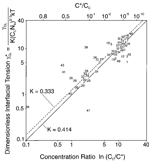
Figure 8.1. Dimensionless interfacial tension \gamma_{CL}^* against the concentration ratio \ln(C_0/C^*) for different K values.
