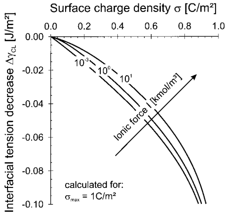
Figure 8.2. Reduction in the interfacial tension \Delta\gamma_{CL} with the surface charge density. Calculated from equation (8.12), valid for \sigma_{\max} = 1 \text{ C/m}^2 . (From Ref. 8.10.)
