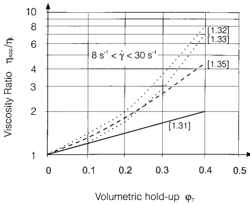
Figure 6.10. Ratio \eta_{\text{app}}/\eta_L versus the volumetric holdup \varphi_T .
