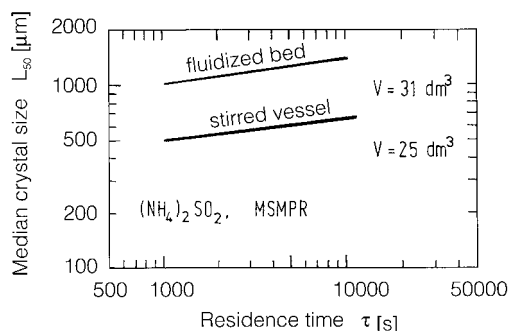
Figure 7.6. Median crystal size of ammonium sulfate in the stirred vessel and fluidized bed.
