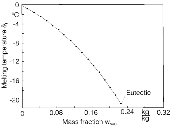
Figure 2.12. Melting temperature versus the mass fraction w_{NaCl} of the system NaCl–H 2 O.
