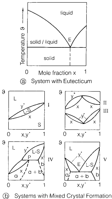
Figure 2.4. Eutectic (a) and noneutectic (b) systems.
