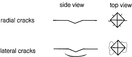
Figure 7.2. Schematic of the observed radial and lateral cracks.
