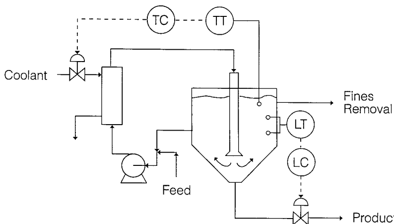
Figure 4.7. Forced-circulation surface-cooled continuous crystallizer.
