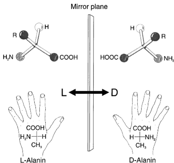
Figure 5.2. The L-form and the D-form of the amino acid alanine.
