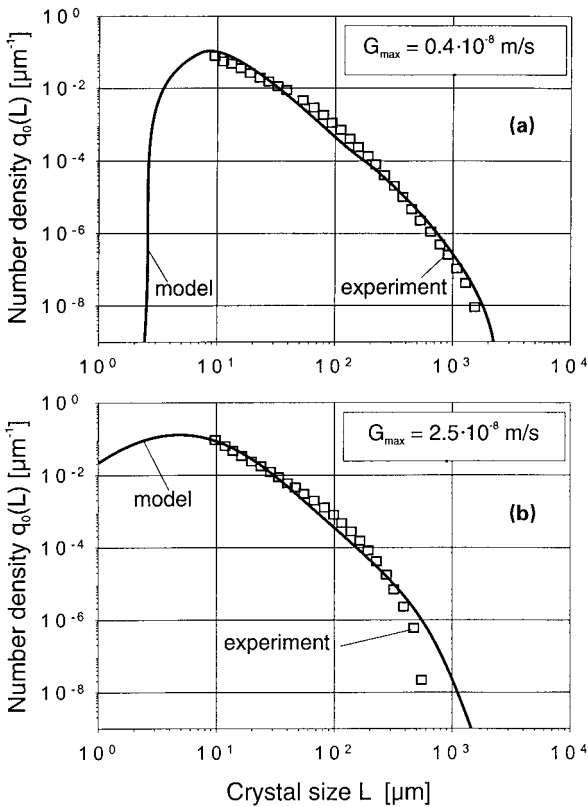
Figure 2.4. Theoretical and experimental number–density distributions from MSMRP experiments. (From Ref. 2.6.)
