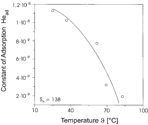
Figure 2.5. Experimentally determined adsorption constant of BaSO 4 on SiO 2 as a function of temperature.
