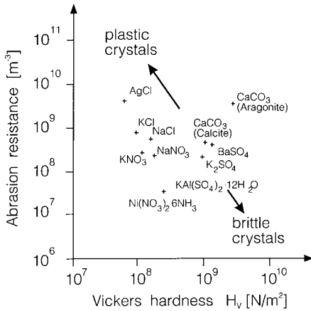
Figure 7.7. Resistance against attrition. (From Ref. 7.8.)
