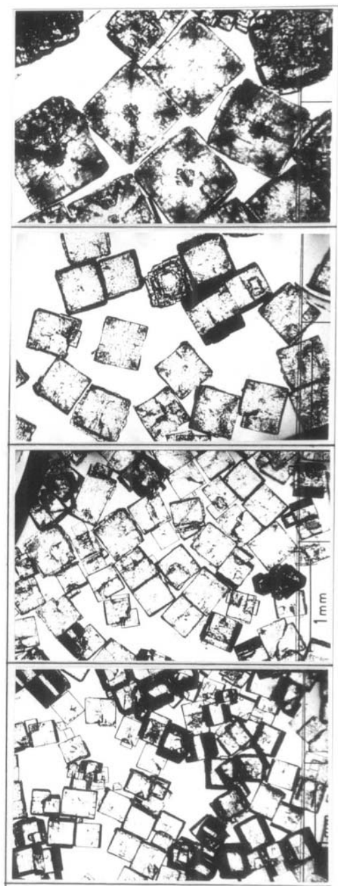
Figure 3.1. Photograph of attrition-resistant potassium chloride crystals.
