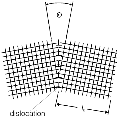
Figure 6.2. Grain-boundary angle between two mosaic blocks.
