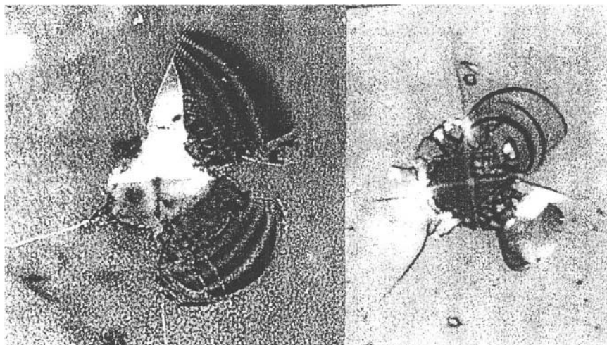
Figure 7.3. Indentations on the \{111\} face of potash alum (left) and the \{101\} face of citric acid (right) at a load of 0.1 N.
