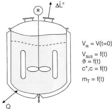
Figure 3.2. Mass balance of a batch crystallizer.
