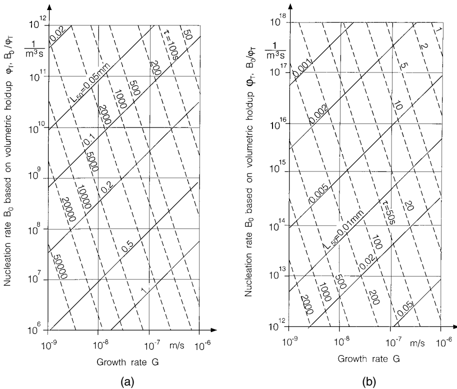
Figure 2.2. Nucleation rate based on volumetric holdup versus crystal growth rate and median crystal size and mean residence time as parameter.
