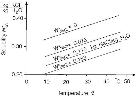
Figure 4.1. Solubility of KCl in the ternary KCl–NaCl–water system.
