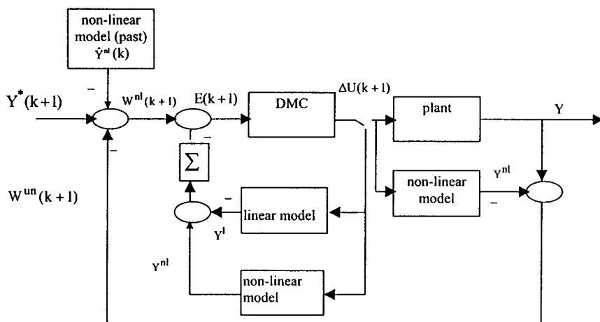
Figure 4.12. Block diagram of the nonlinear quadratic dynamic matrix controller for the control of the 1-m 3 crystallizer. K : sampling interval, Y : process output, Y^l : output of the linear model, Y^{nl} : output of the nonlinear model, E : the error signal, Y^* : the set point, W = Y - Y^{nl} .
