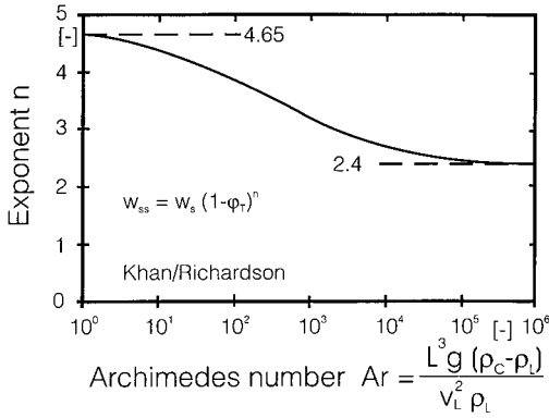
Figure 6.8. Exponent n as function of the Archimedes number.
